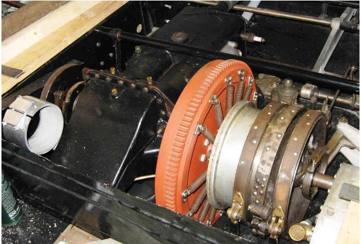
Trojan engine and epicyclic gearbox installed
